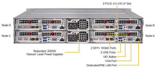
(Rear View – System)
